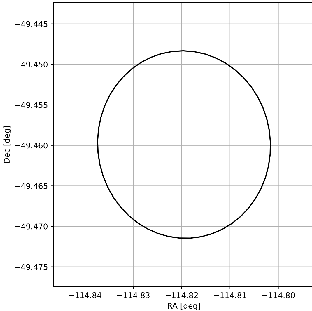
4FGL J1620.7-4927
