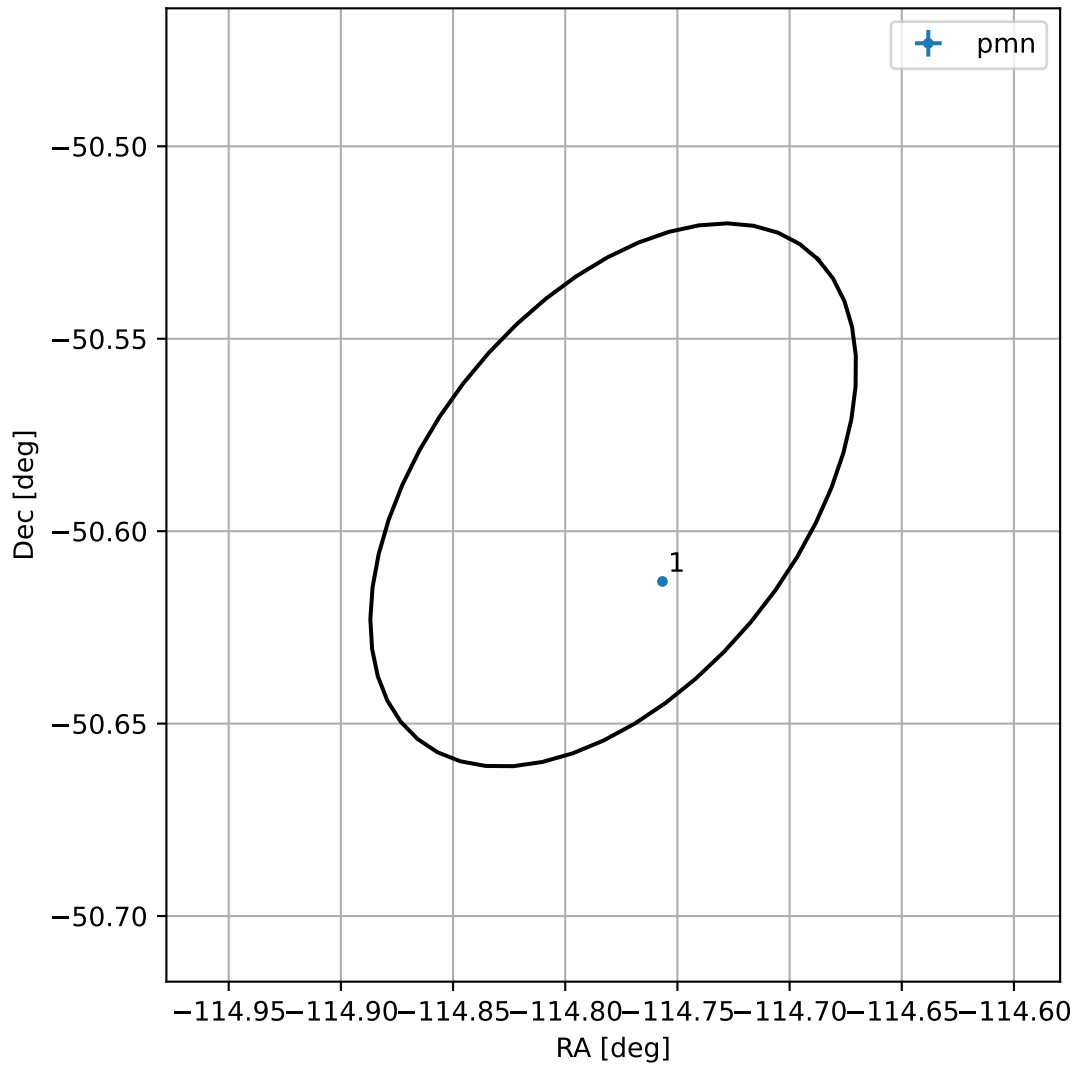
4FGL J1620.8-5035
