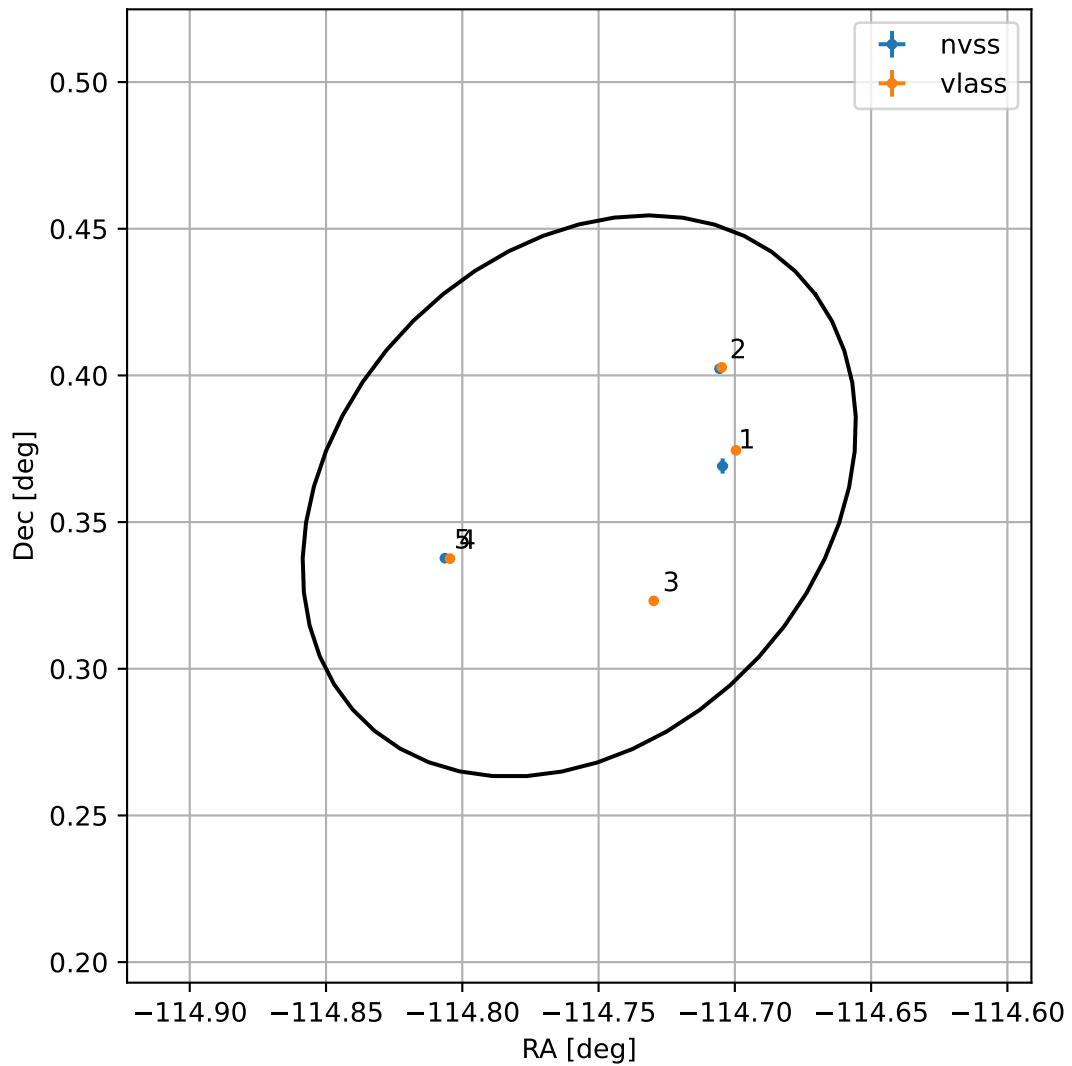
4FGL J1620.9+0021
