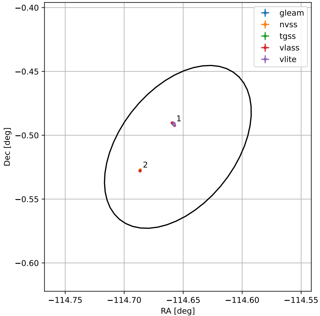
4FGL J1621.3-0030
