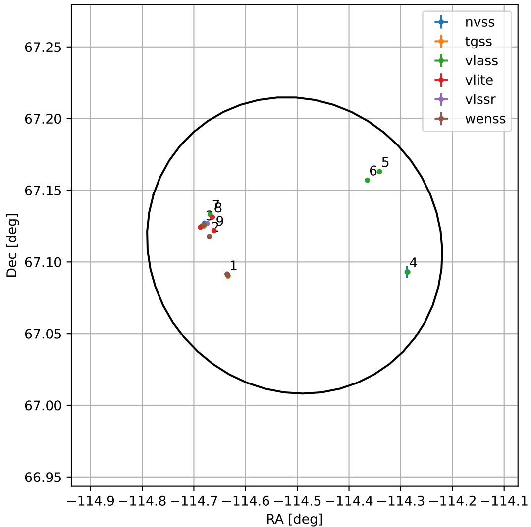
4FGL J1621.9+6706
