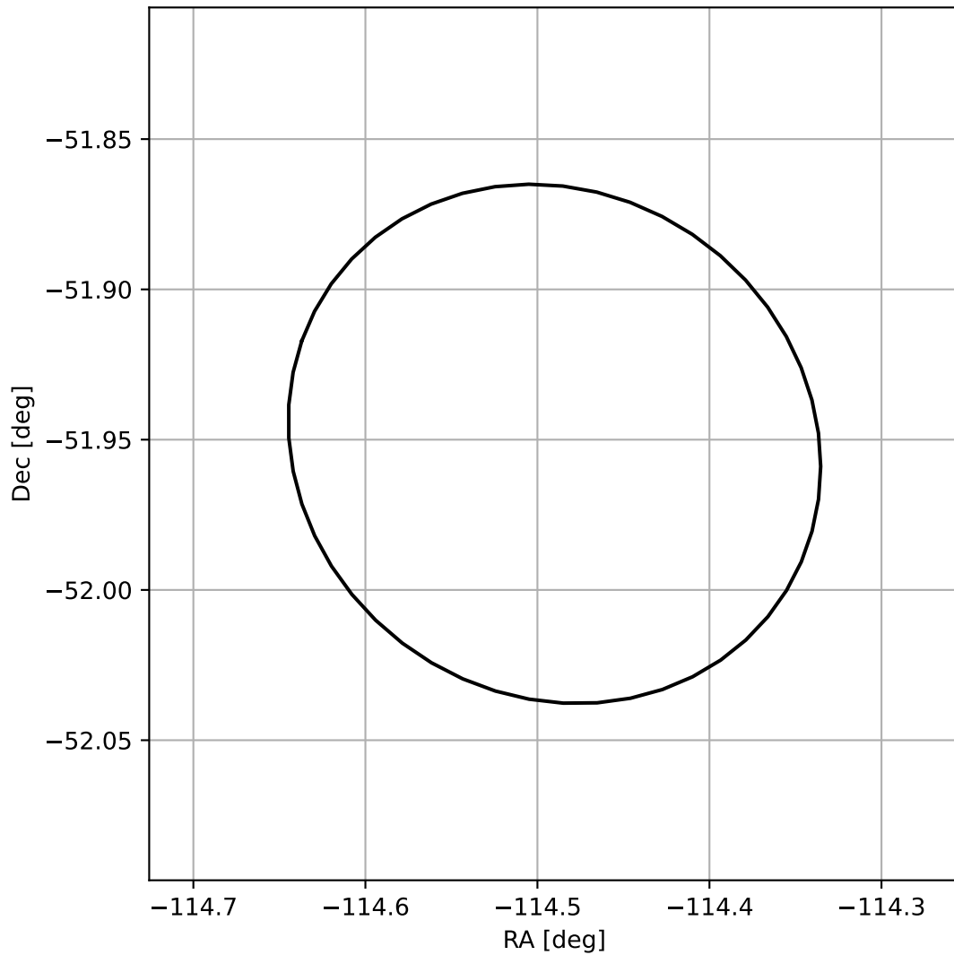
4FGL J1622.0-5157
