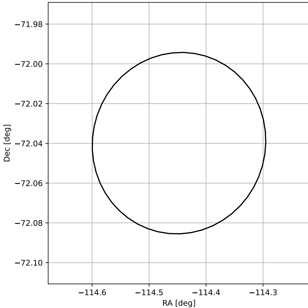
4FGL J1622.2-7202
