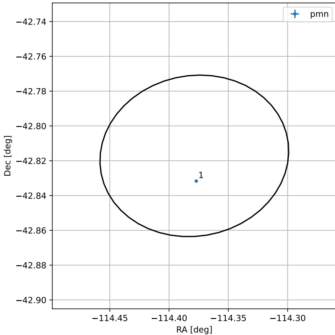
4FGL J1622.4-4249
