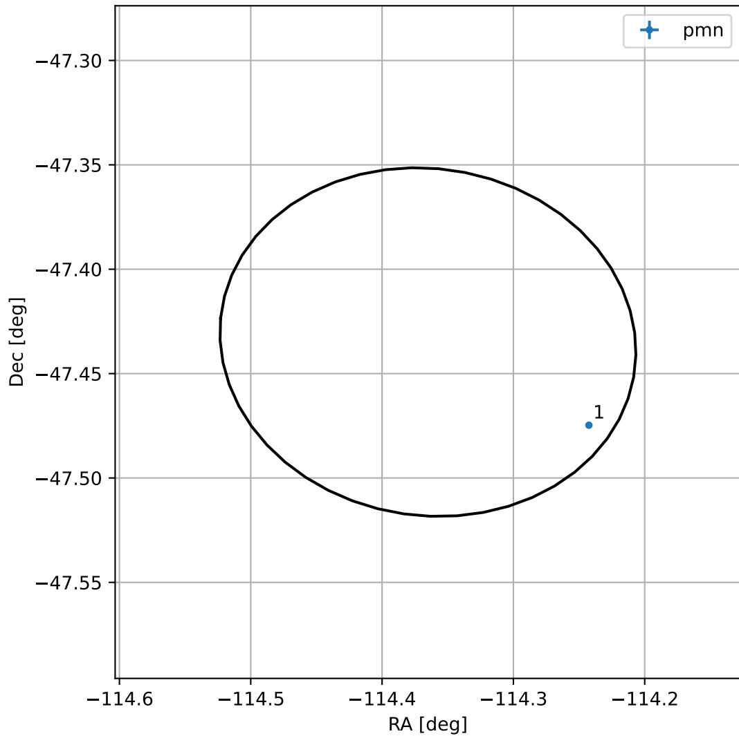
4FGL J1622.5-4726
