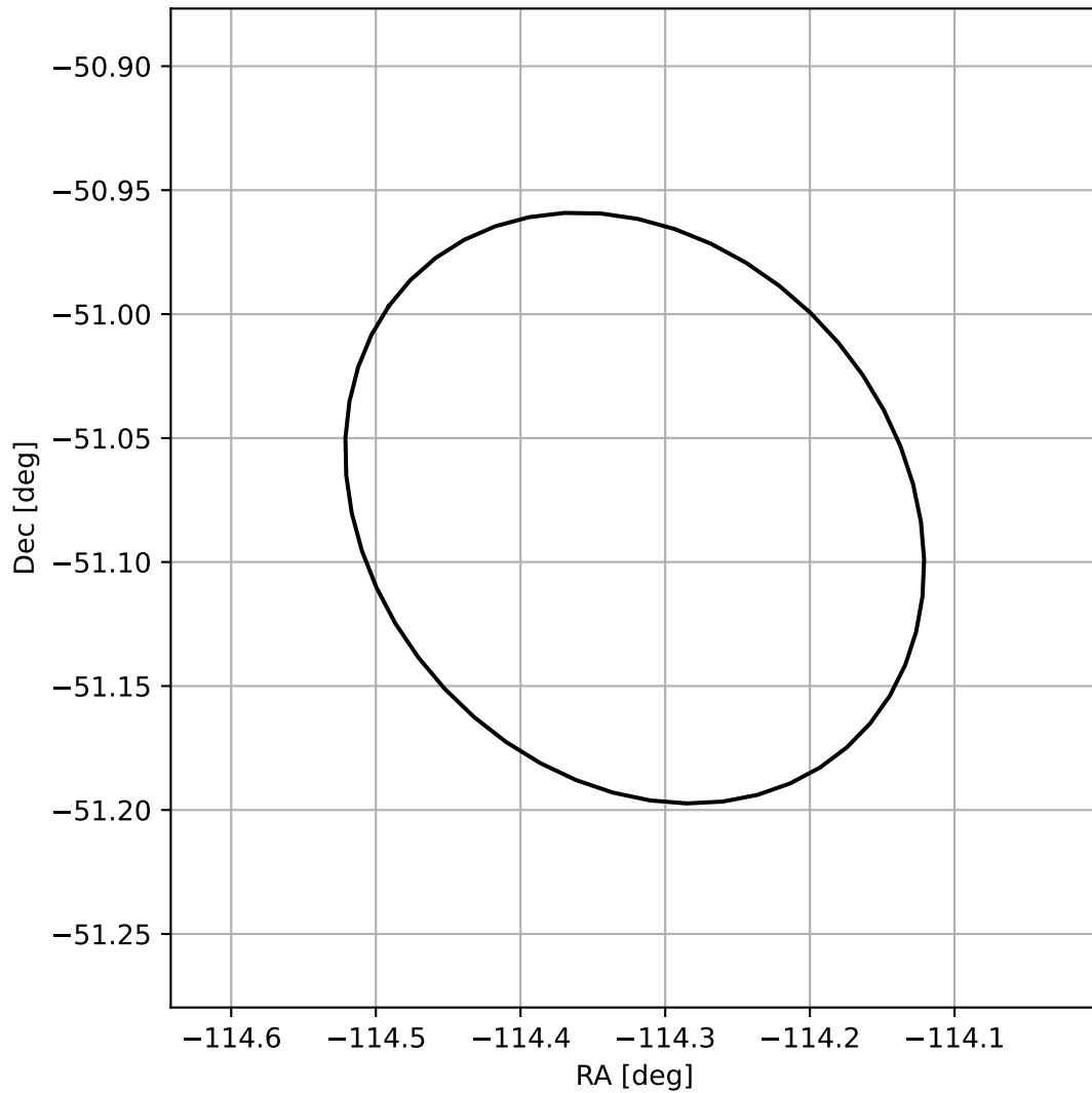
4FGL J1622.7-5104
