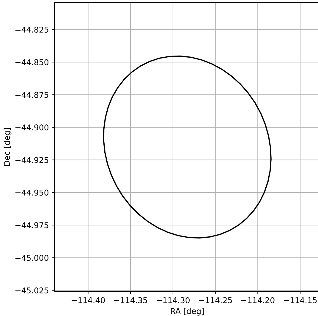
4FGL J1622.8-4454
