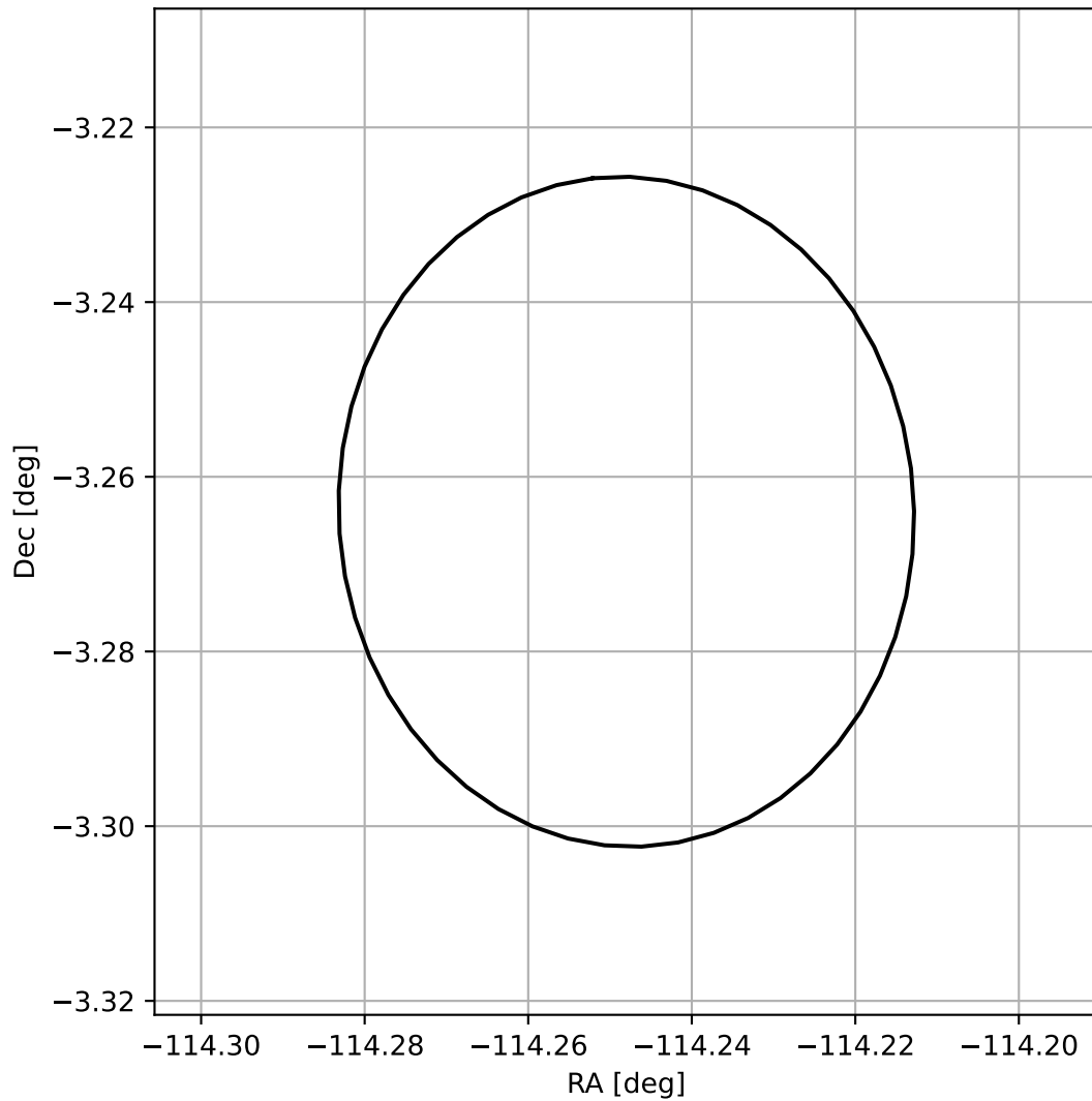
4FGL J1623.0-0315
