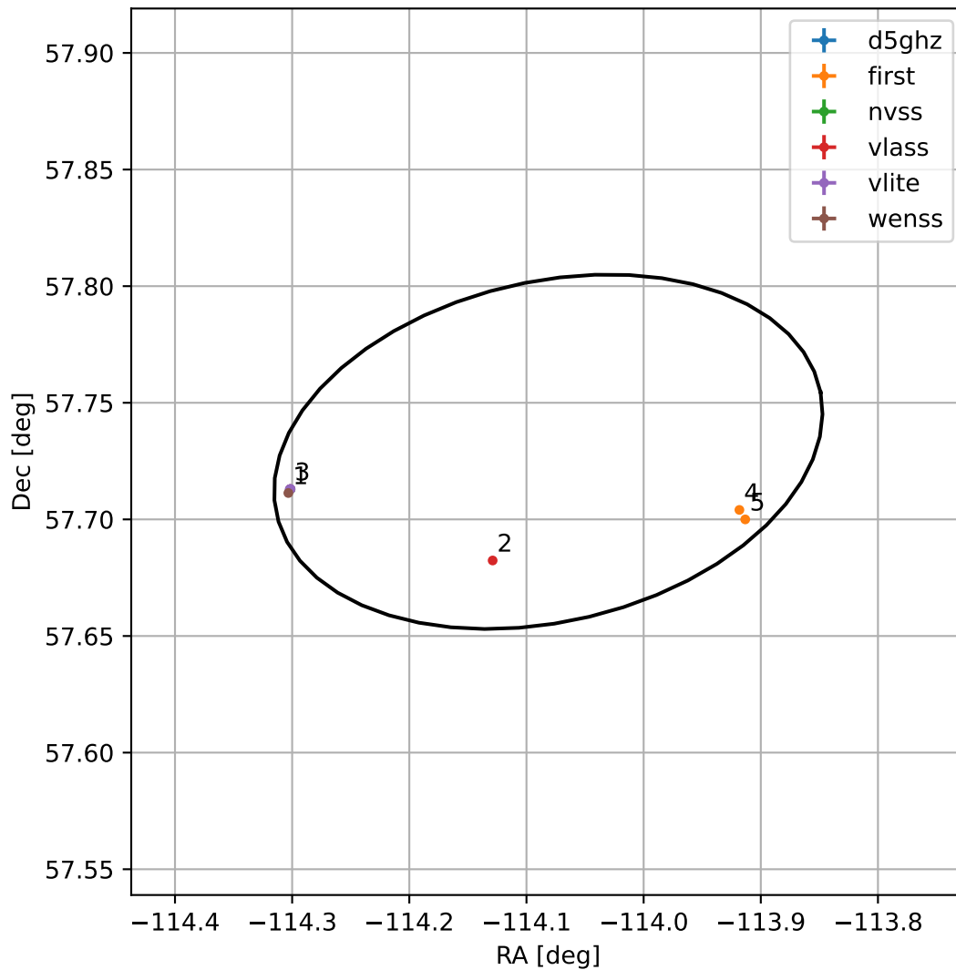
4FGL J1623.6+5743
