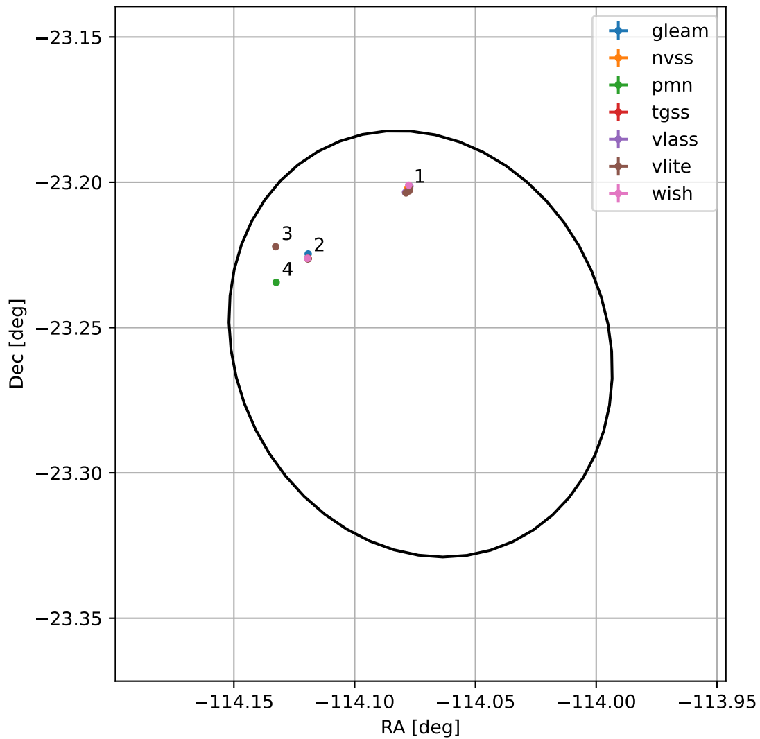
4FGL J1623.7-2315
