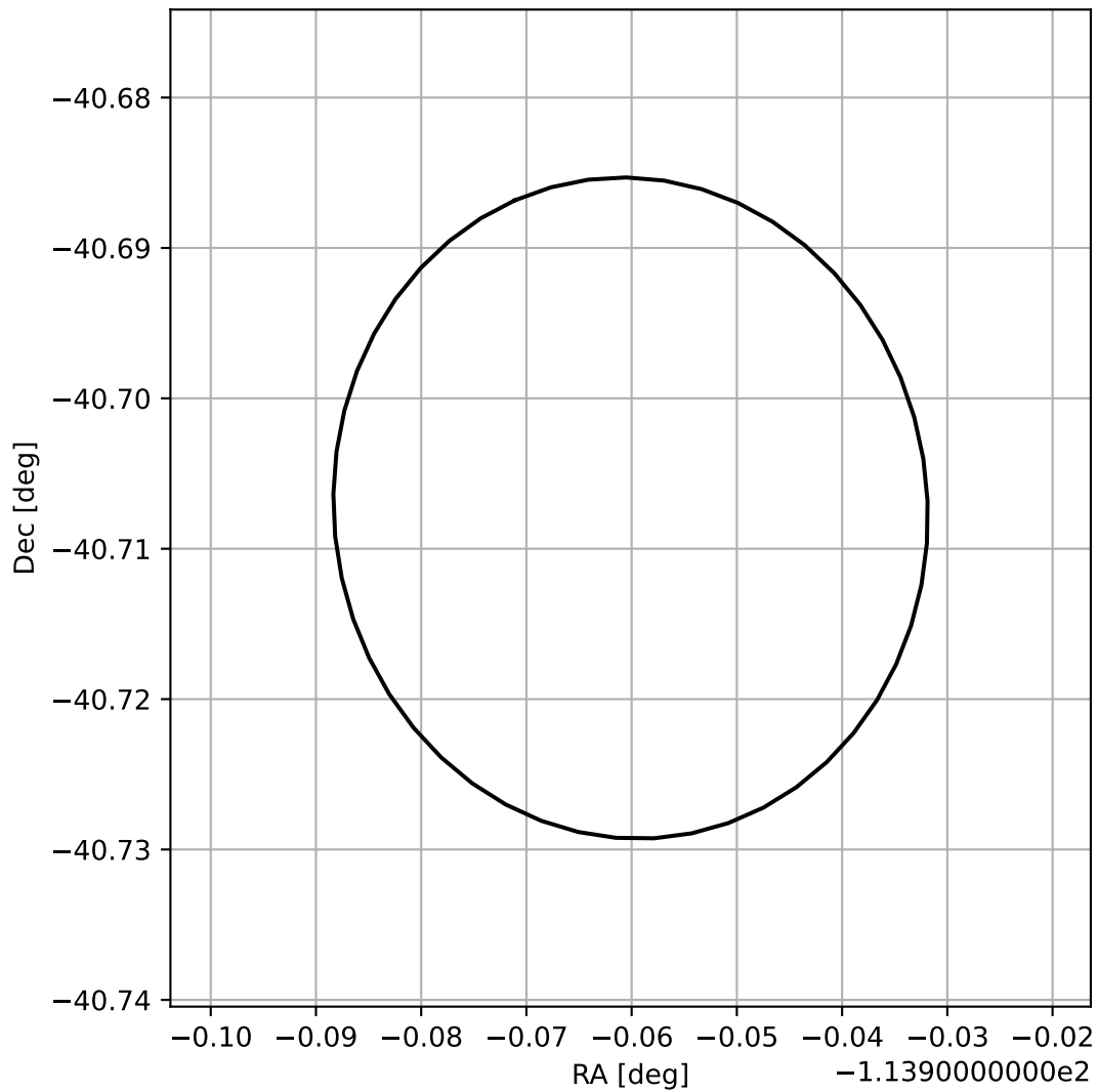
4FGL J1624.1-4042
