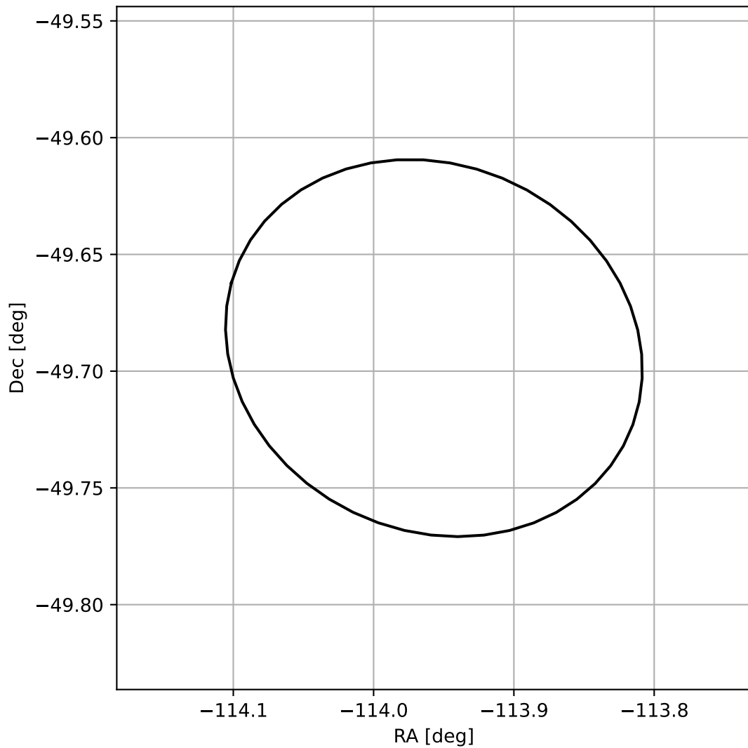
4FGL J1624.1-4941
