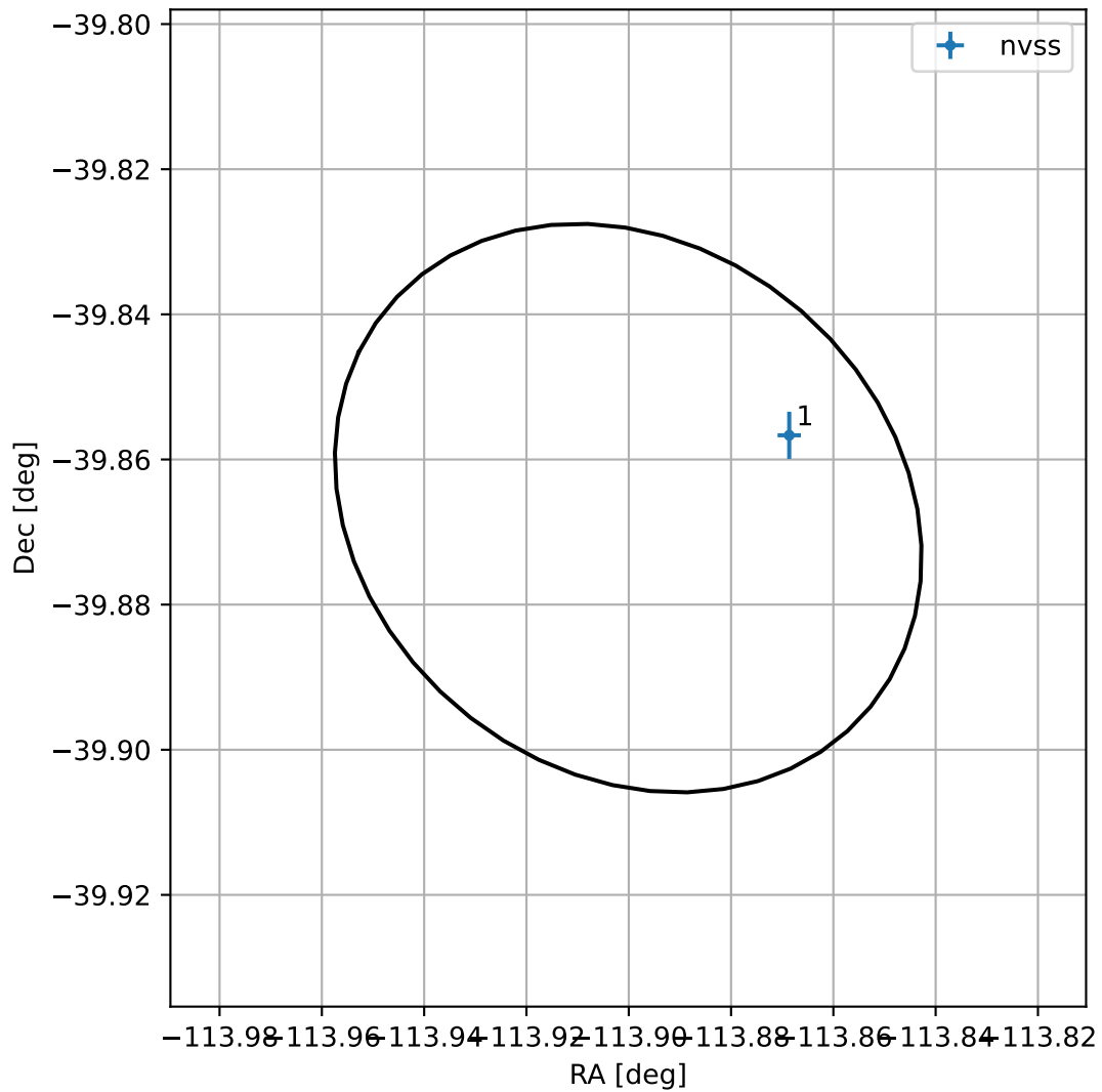
4FGL J1624.3-3952
