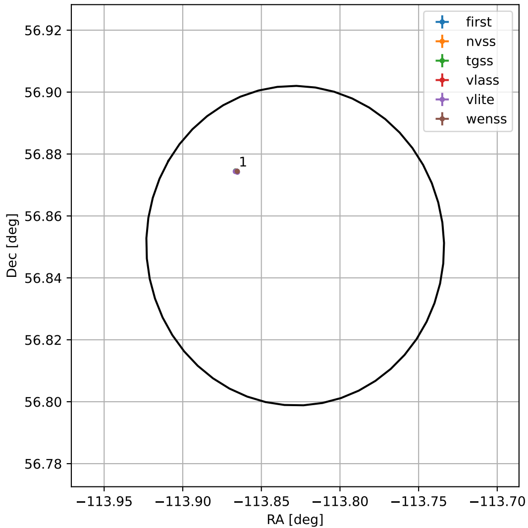
4FGL J1624.6+5651
