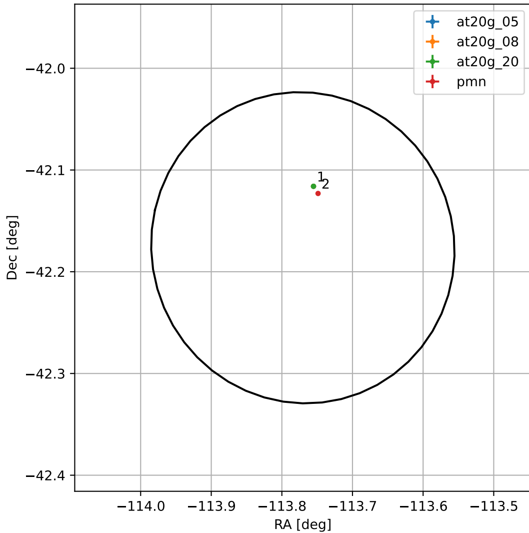
4FGL J1624.9-4210
