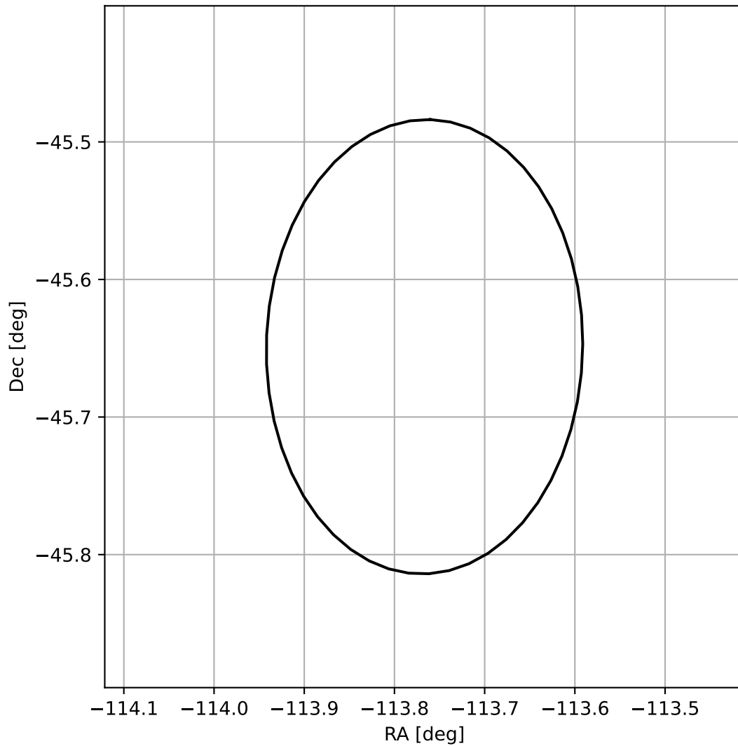
4FGL J1624.9-4538
