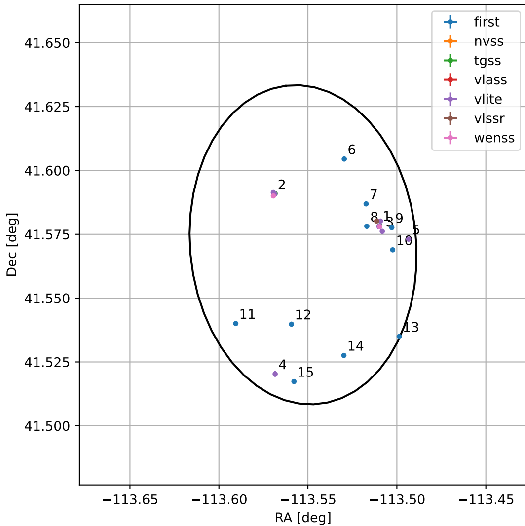
4FGL J1625.7+4134
