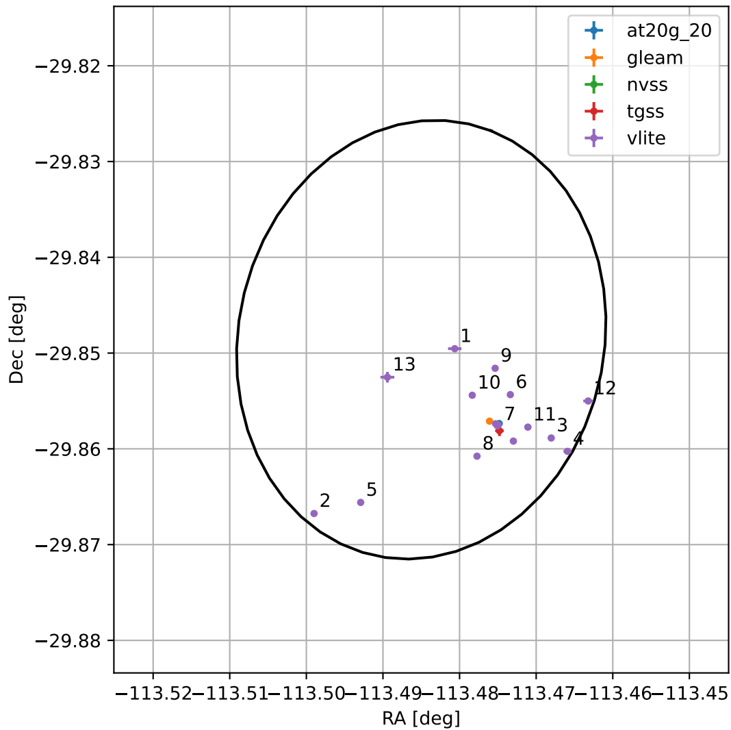
4FGL J1626.0-2950
