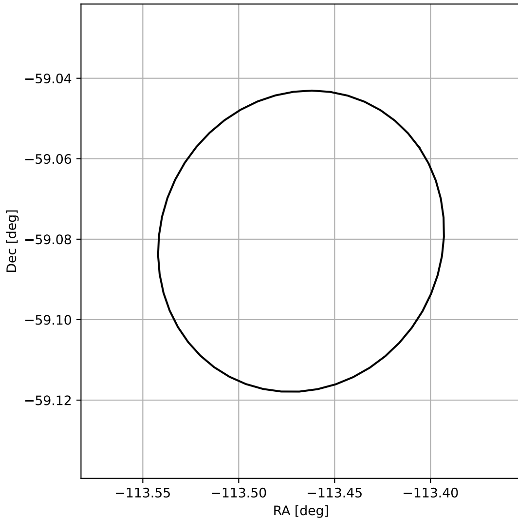
4FGL J1626.1-5904
