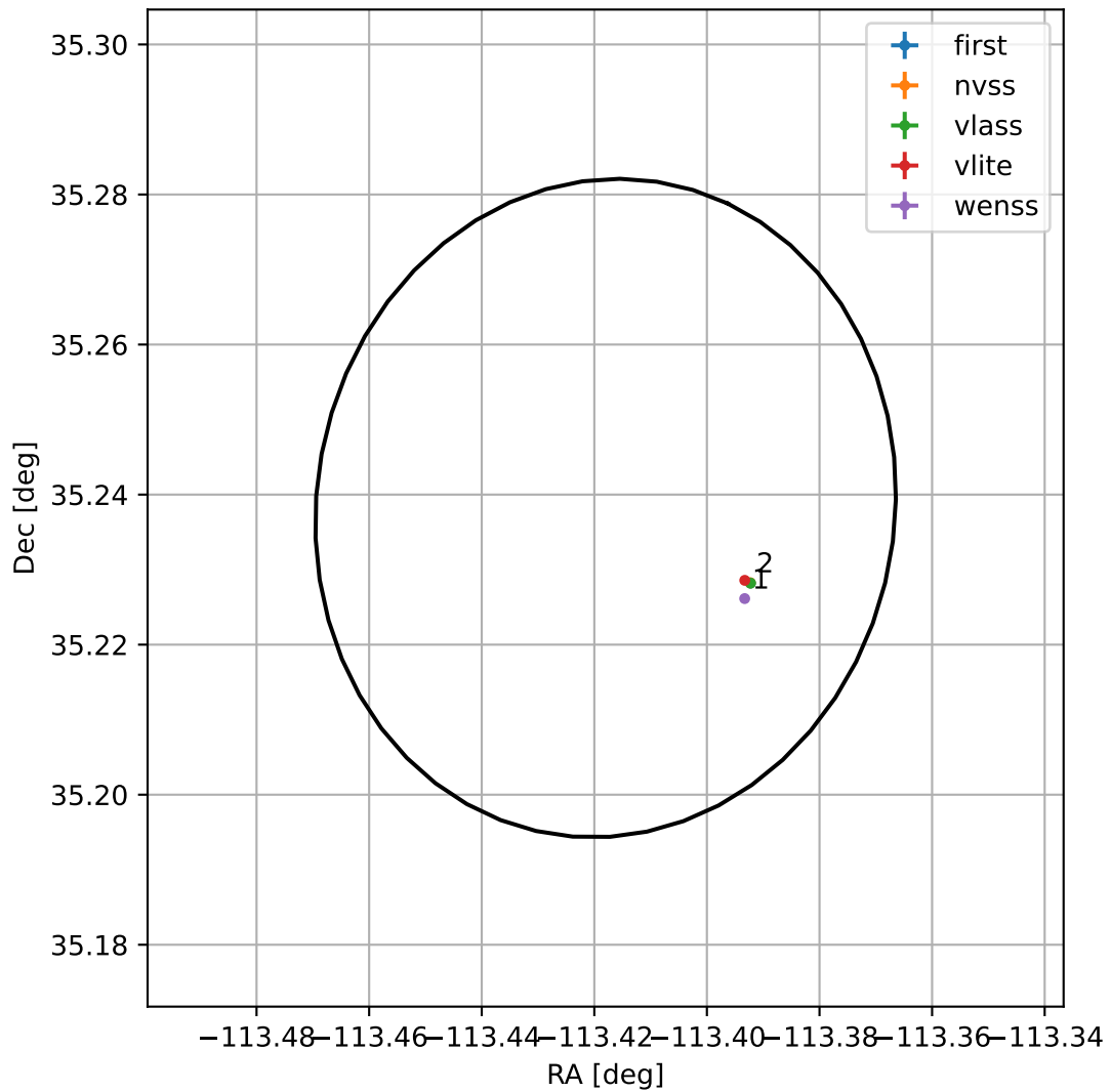
4FGL J1626.3+3514
