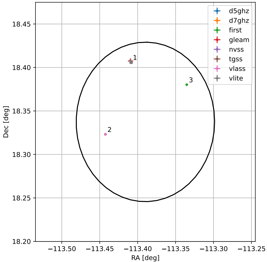
4FGL J1626.4+1820
