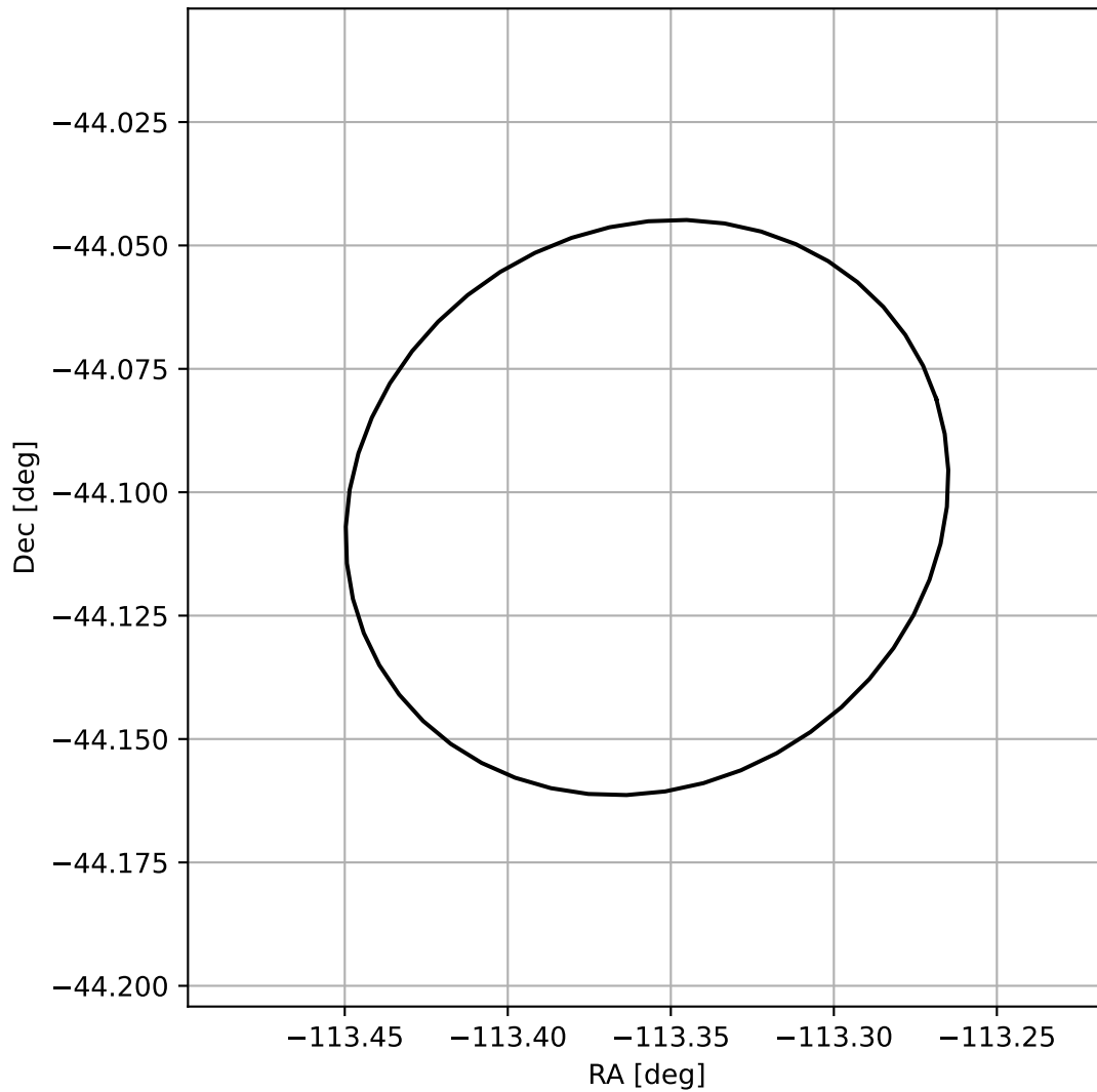
4FGL J1626.5-4406
