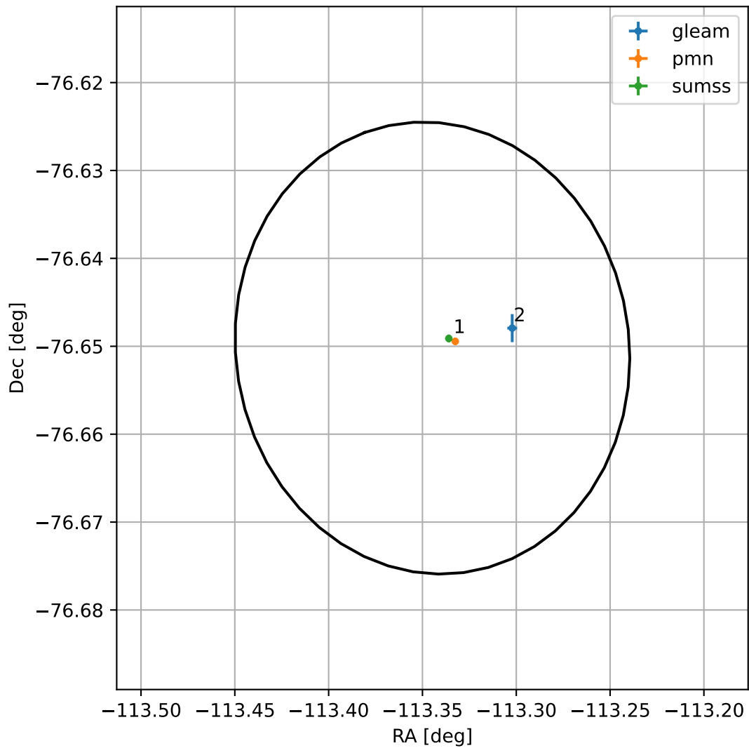
4FGL J1626.6-7639
