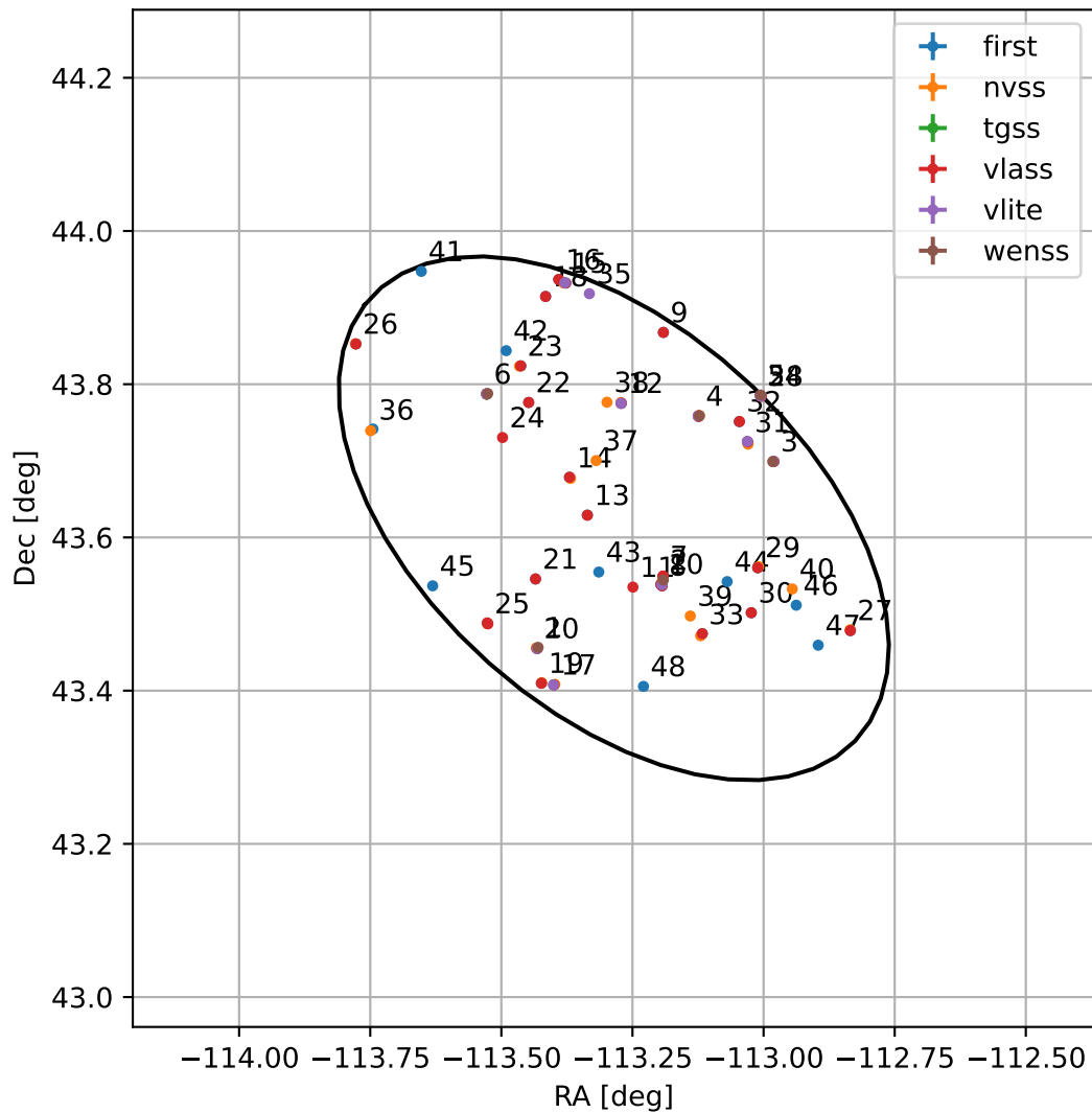
4FGL J1626.8+4337
