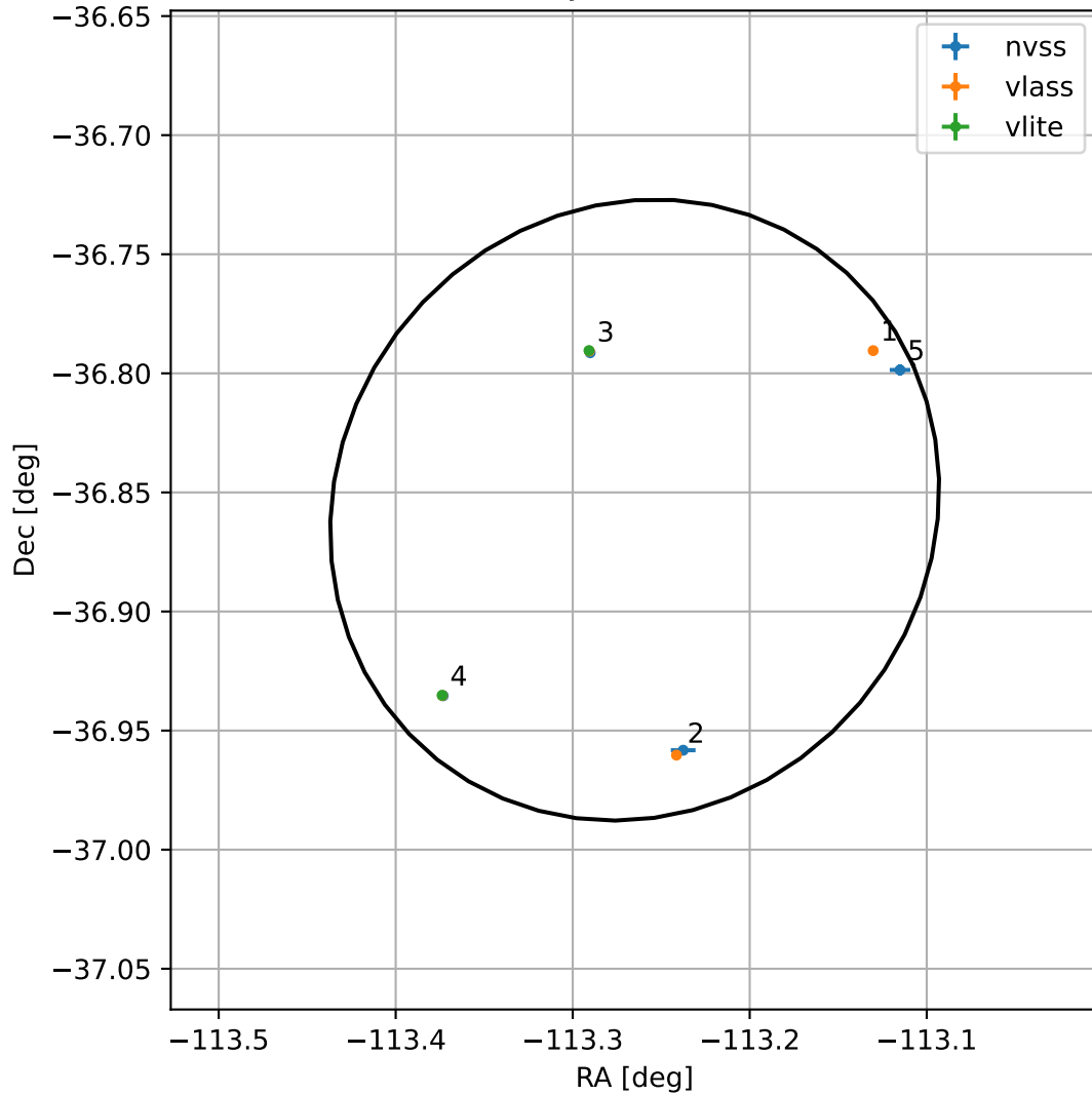
4FGL J1626.9-3651
