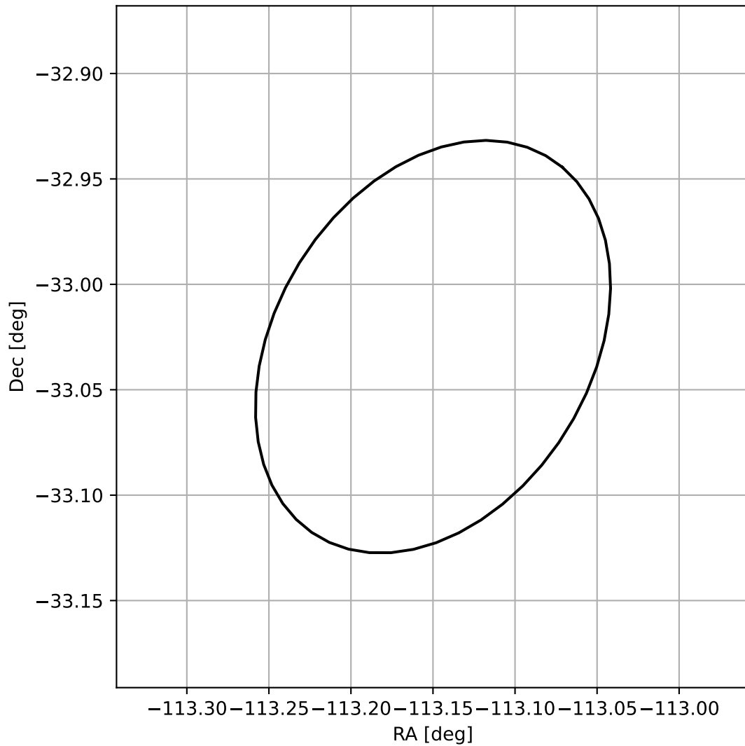
4FGL J1627.4-3301
