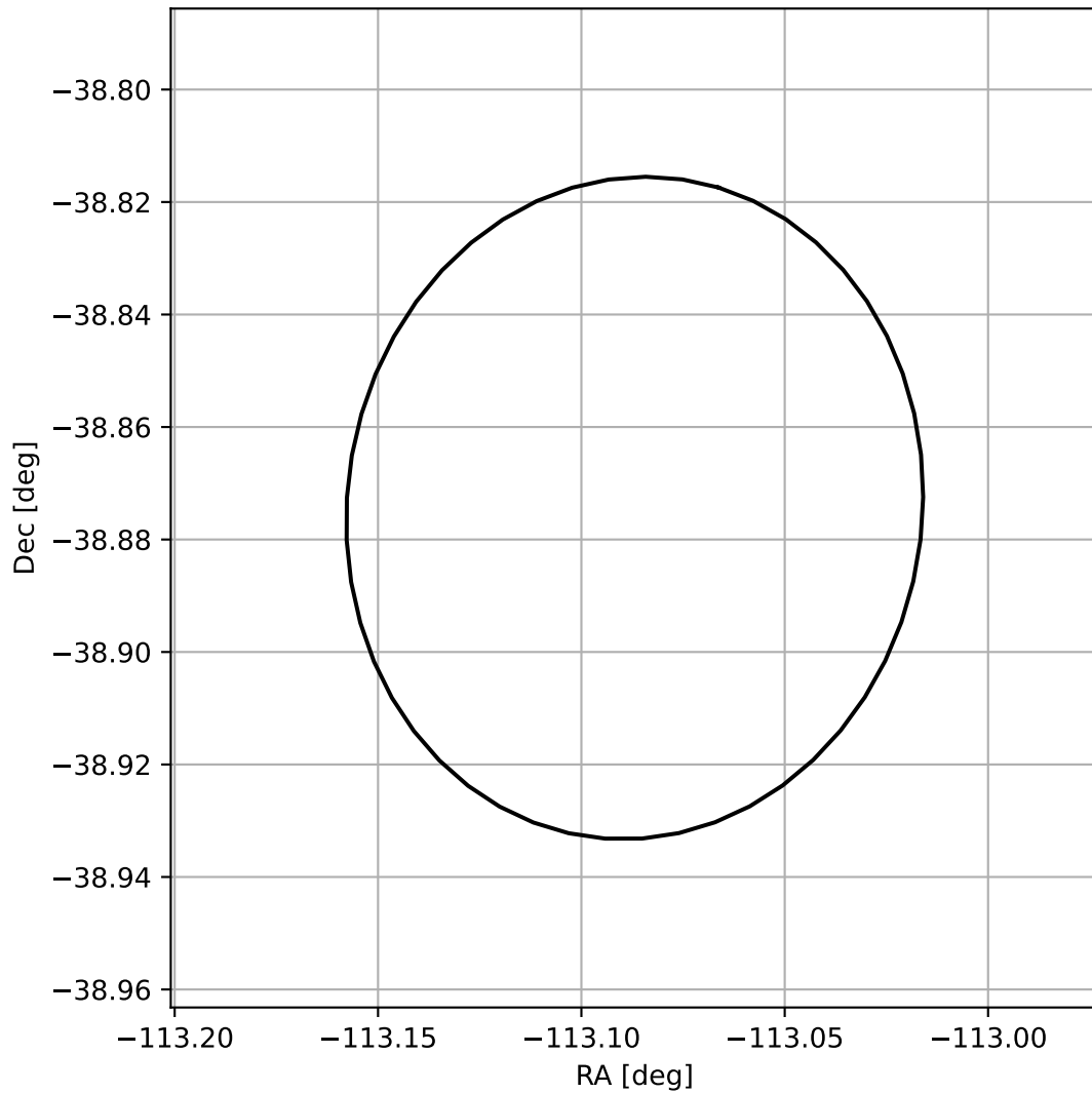
4FGL J1627.6-3852
