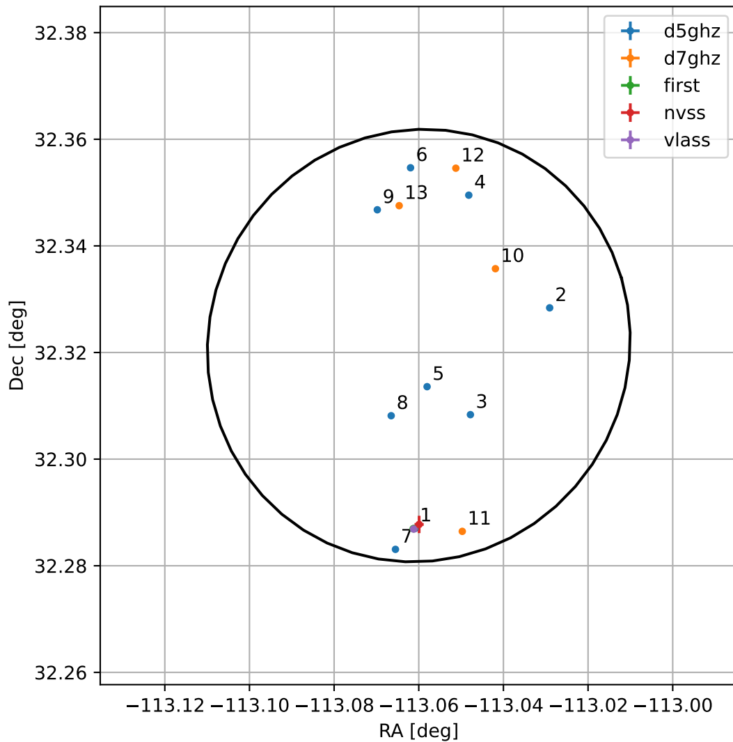
4FGL J1627.7+3219
