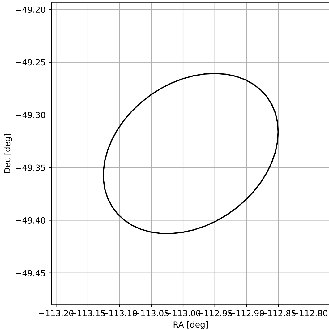
4FGL J1628.0-4920
