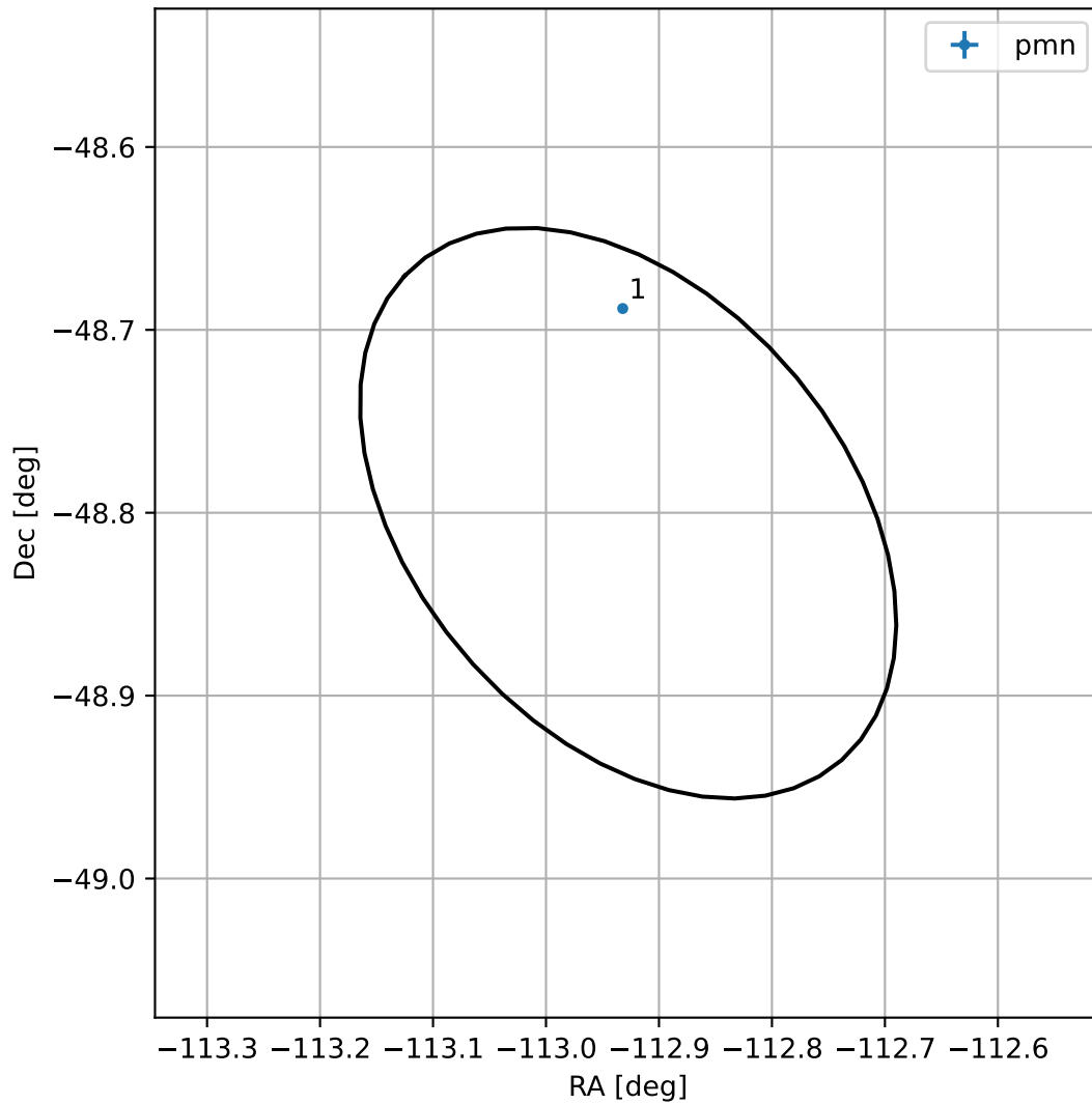
4FGL J1628.2-4848
