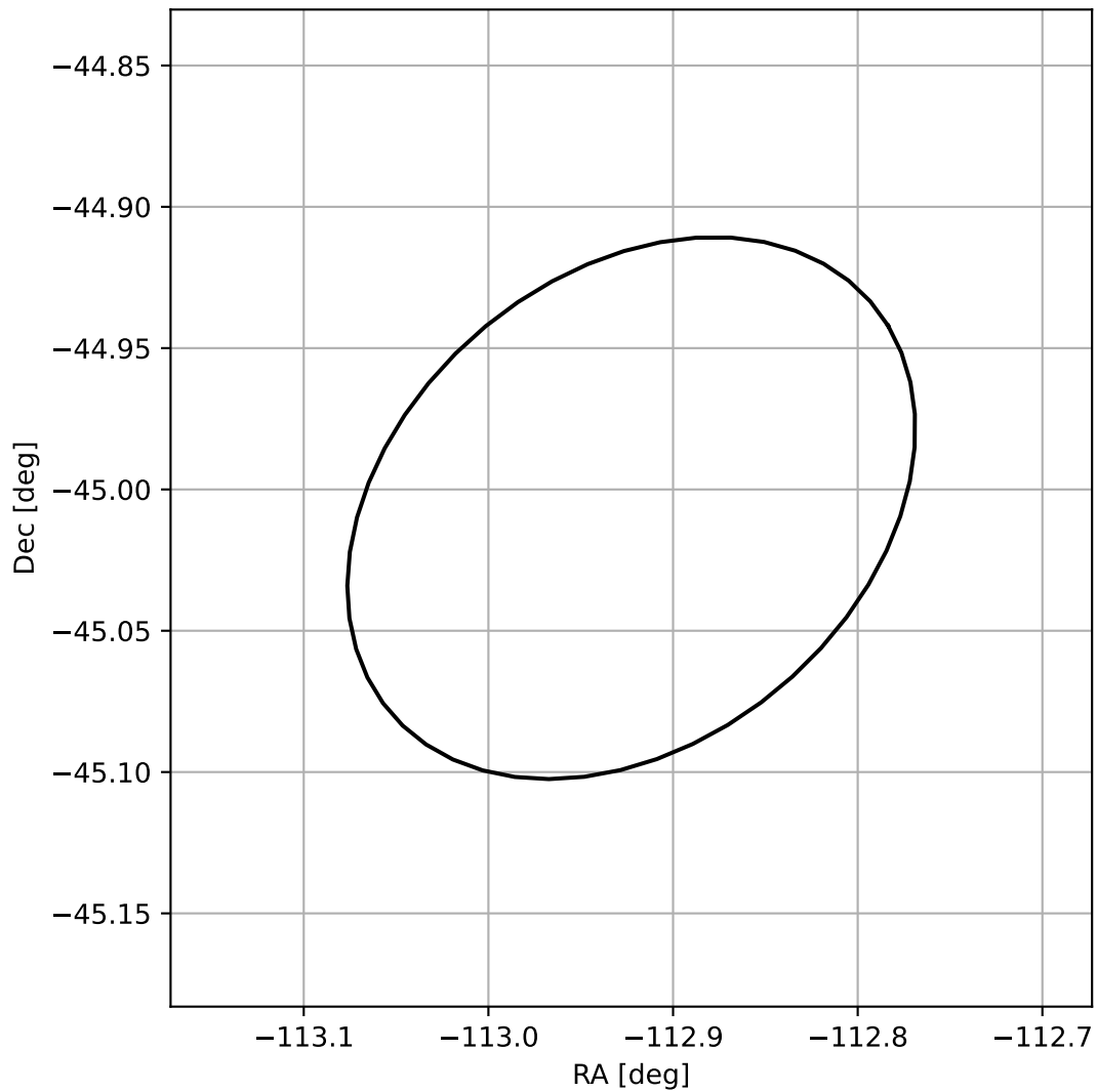
4FGL J1628.3-4500
