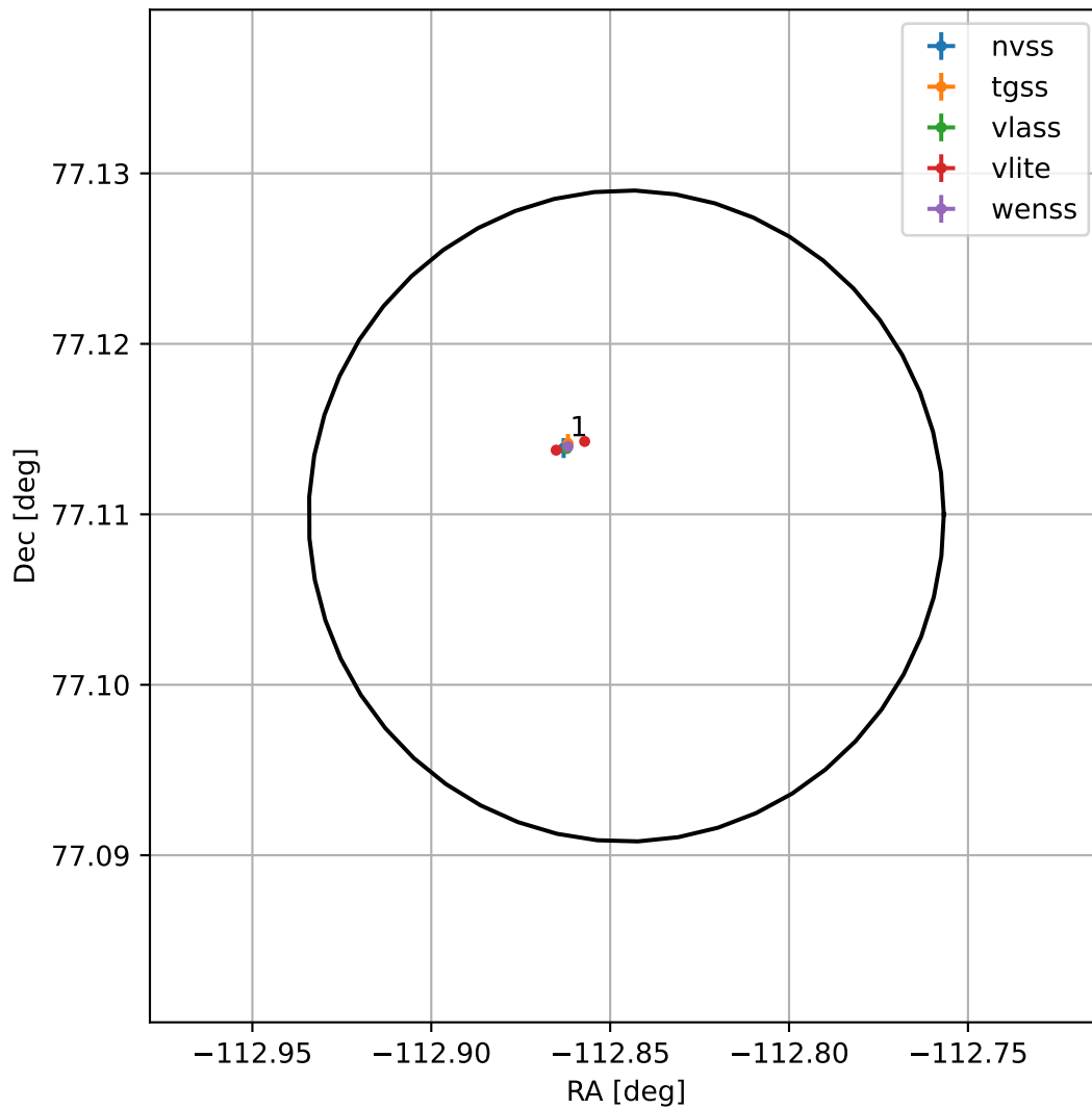
4FGL J1628.6+7706
