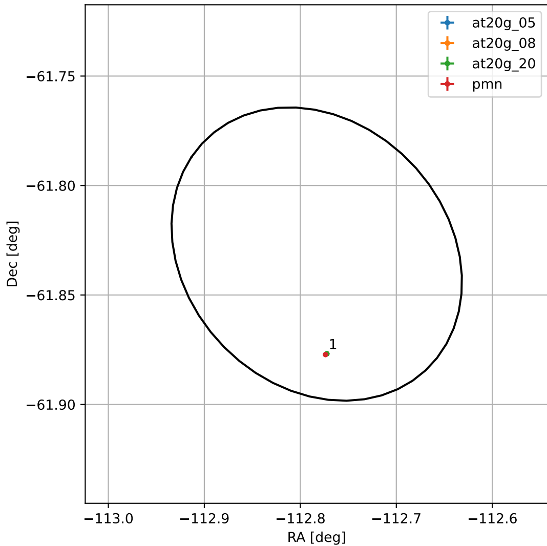
4FGL J1628.8-6149
