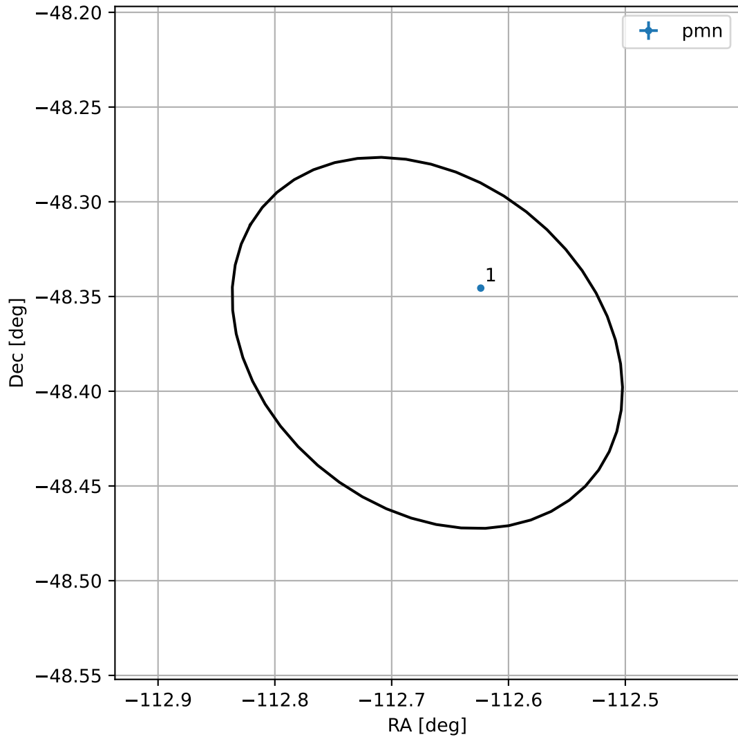
4FGL J1629.3-4822
