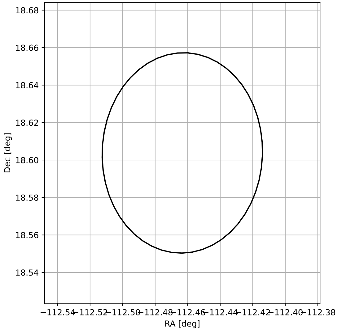
4FGL J1630.1+1836
