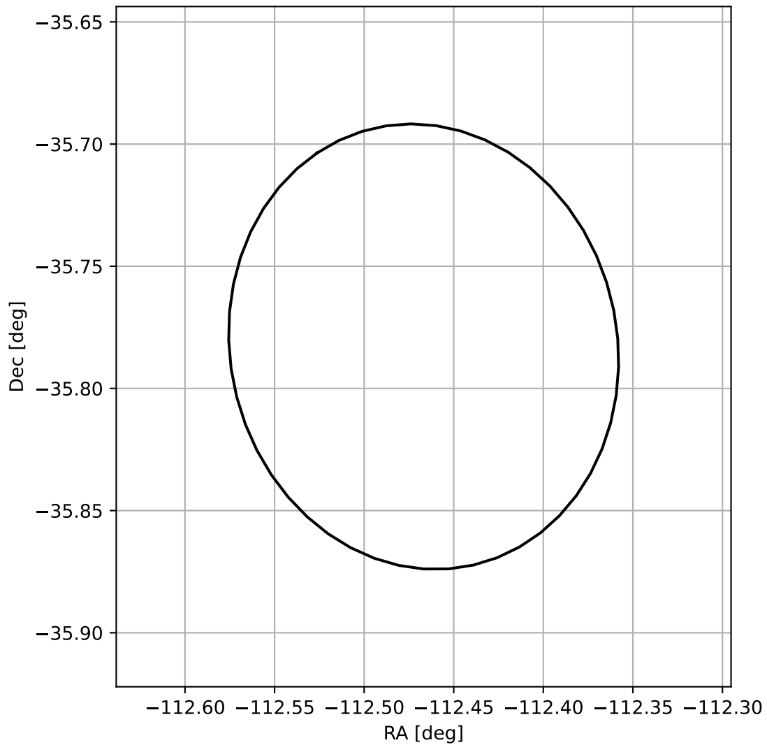
4FGL J1630.1-3546
