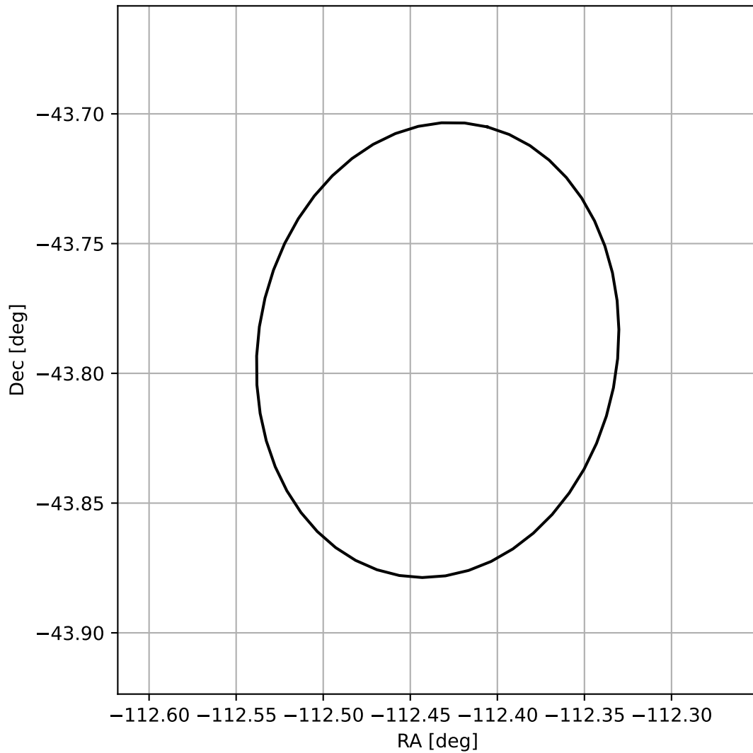
4FGL J1630.2-4347
