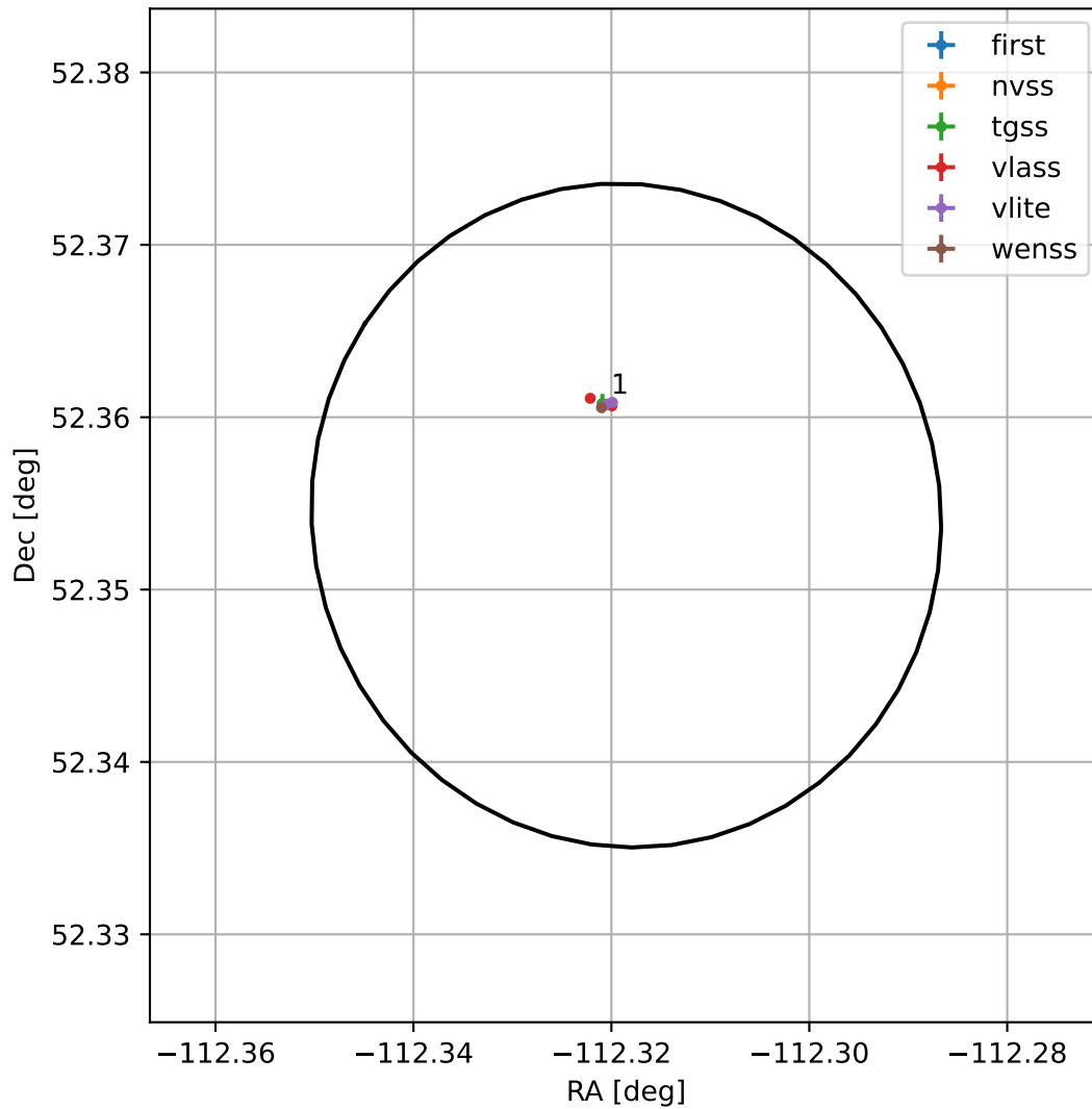
4FGL J1630.7+5221
