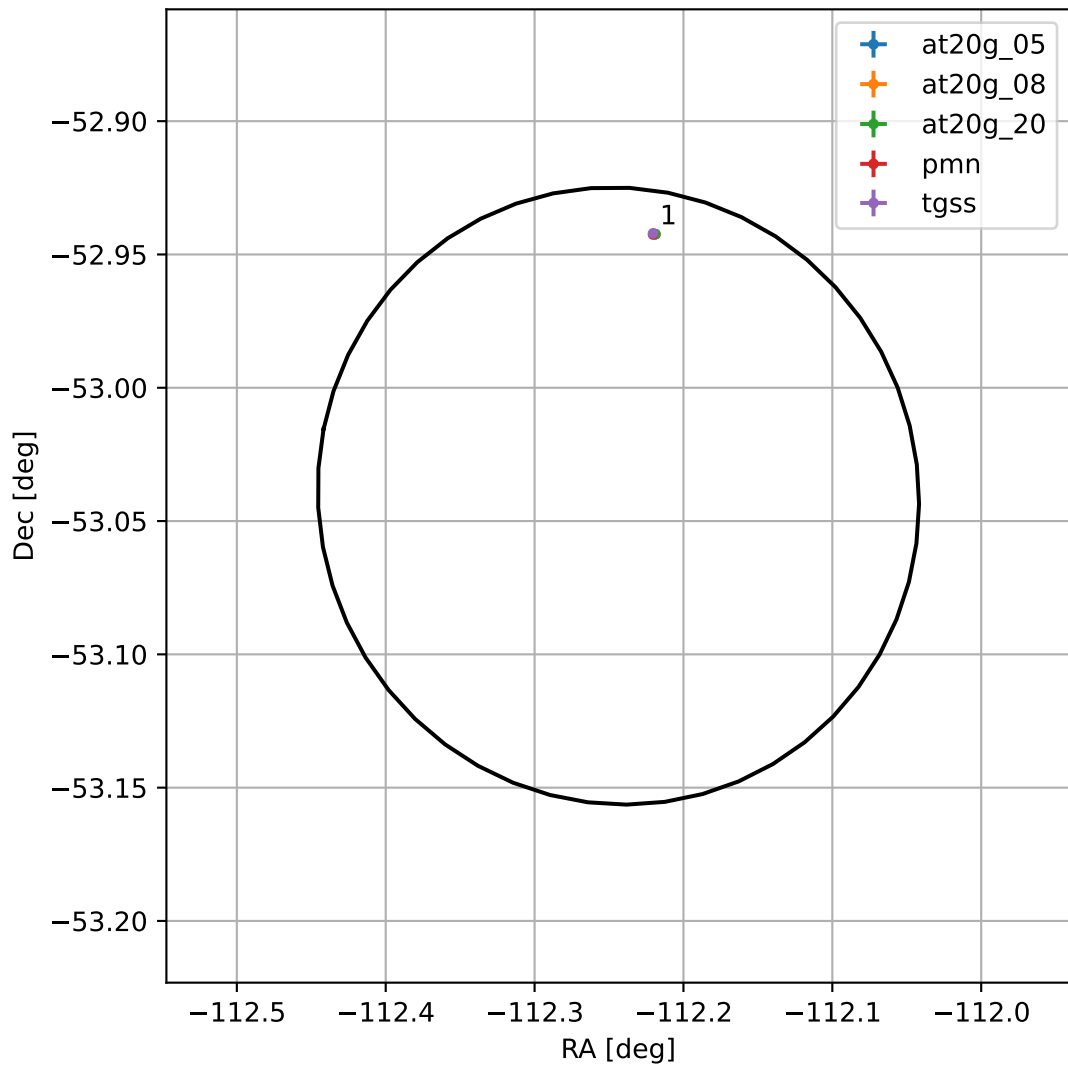
4FGL J1631.0-5302
