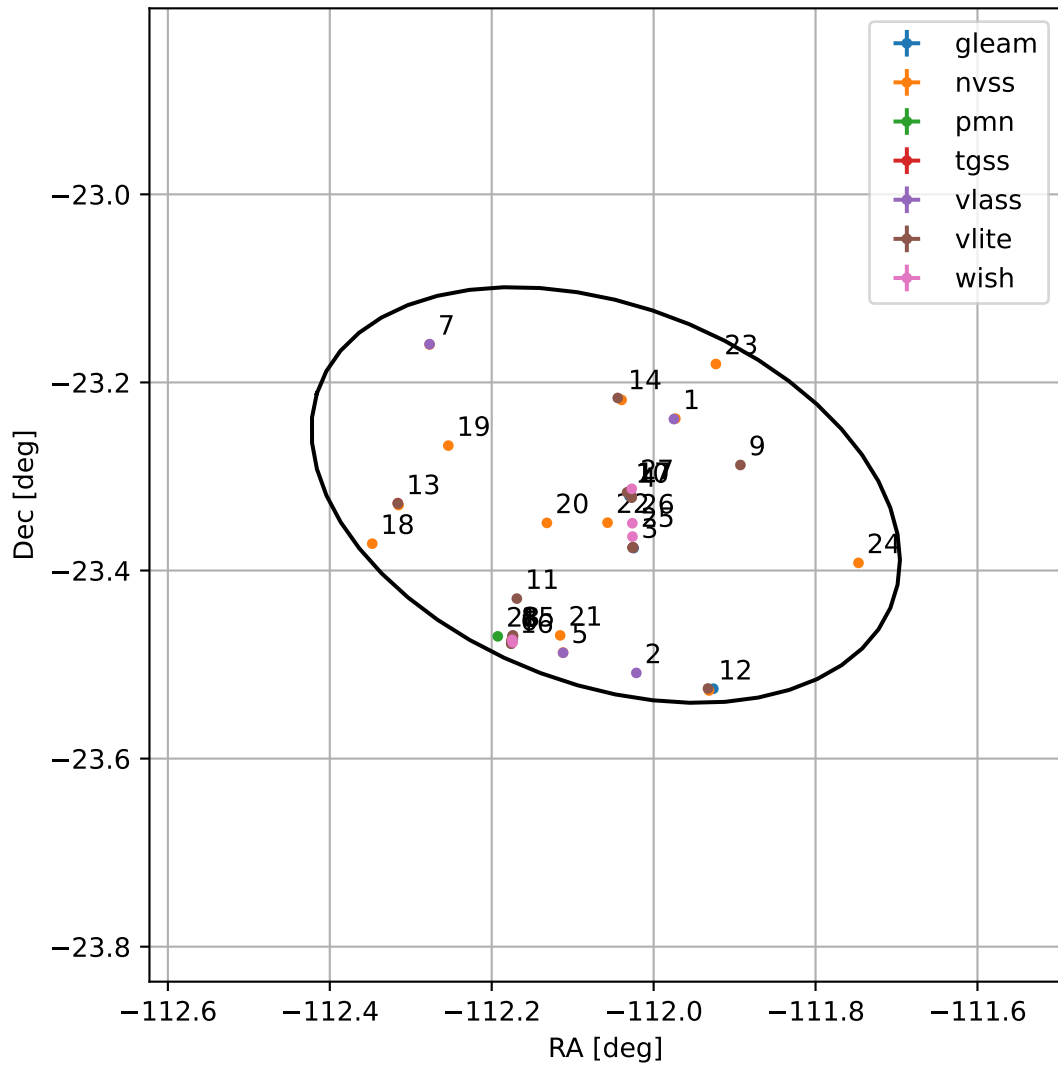
4FGL J1631.7-2319
