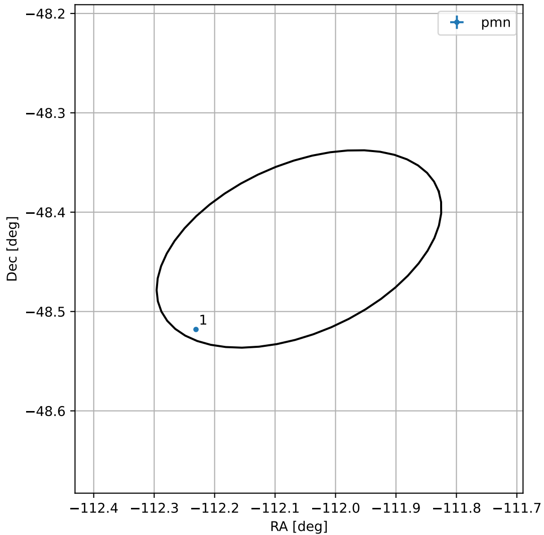
4FGL J1631.7-4826
