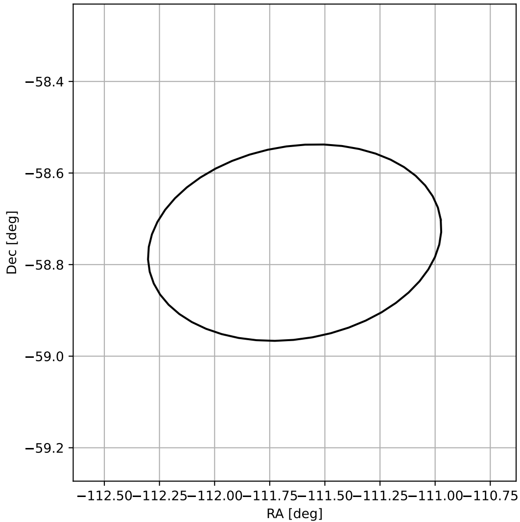
4FGL J1633.4-5845
