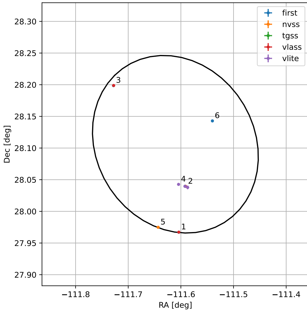
4FGL J1633.5+2806
