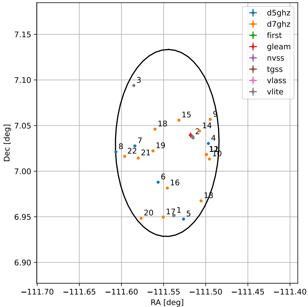
4FGL J1633.8+0701
