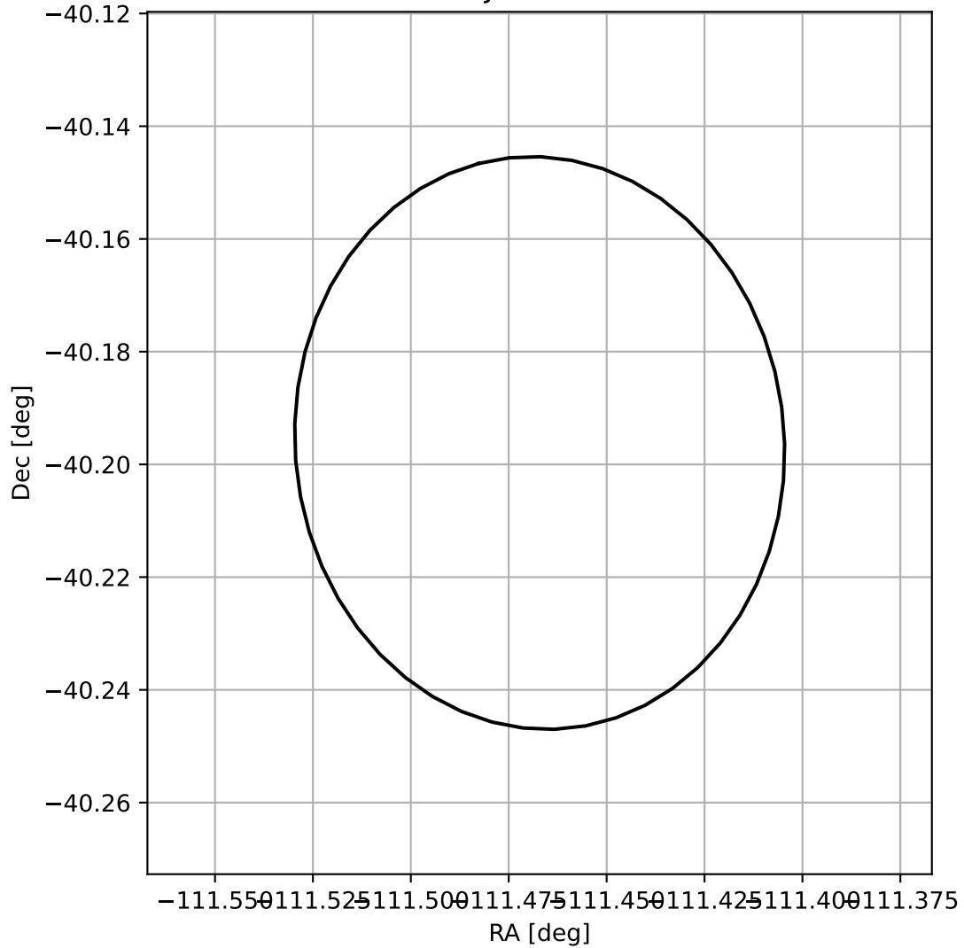
4FGL J1634.1-4011
