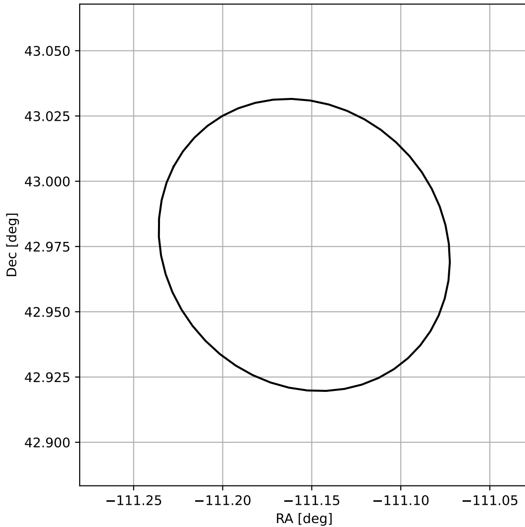
4FGL J1635.3+4258
